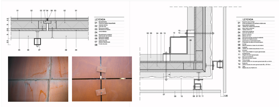
Figure 3: Construction plan detailing restored original facade.
