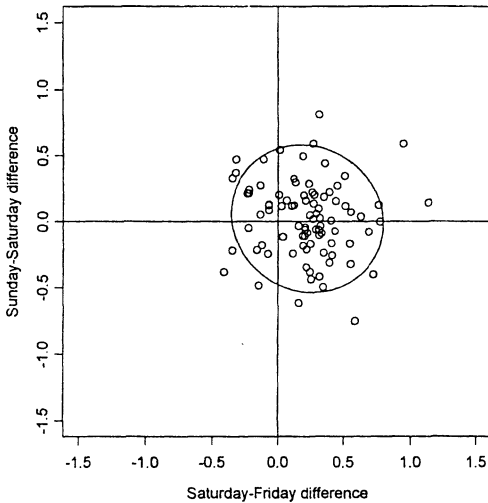
Figure 4: Scatter plot of Sunday-Saturday vs. Saturday-Friday differences for Azusa, 1994-97. The ellipse, in this case nearly circular, includes roughly the inner 95% of the data points for a normal distribution.
