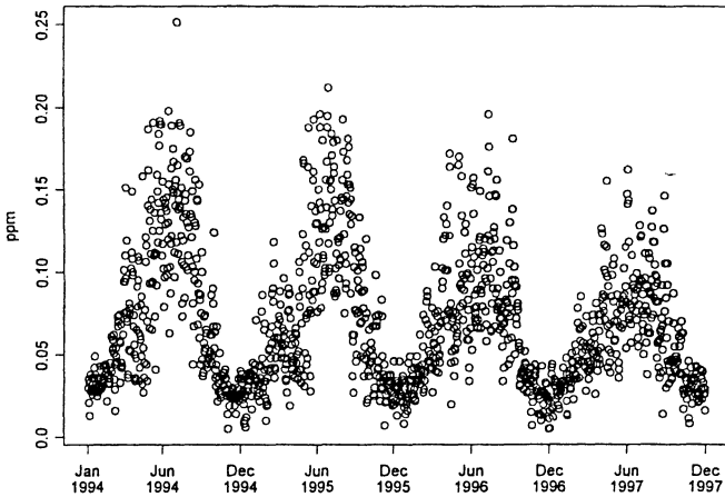
Figure 2: Daily peak ozone concentration, Azusa, 1994-97.
