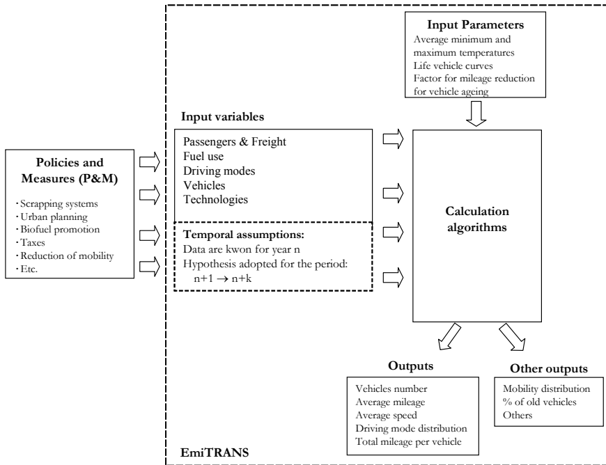
Figure 2: EmiTRANS design.
